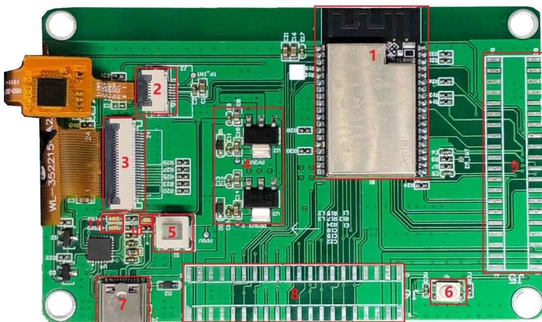
Figure 3: The Back of the Physical Drawing of the WT32-SC01
